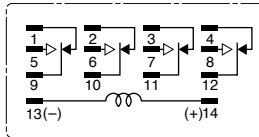
4PDT (RY4/RM42)
