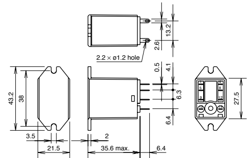
RM2S-UT
