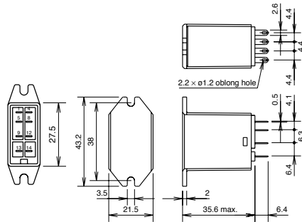
RY4S-UT/RY42S-UT
