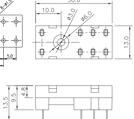
SQ2V-63
