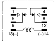
DPDT Wide (RM2)
