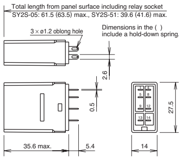
RY2S/RY22S
