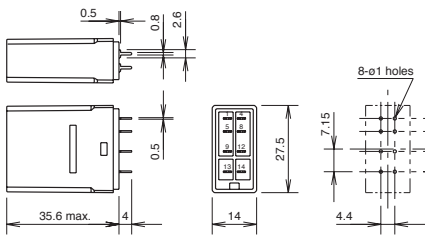
RY2V/RY22V
